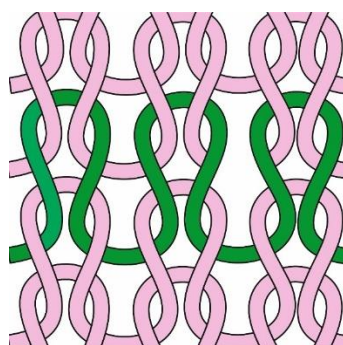
Figure 1.14: Plain Knit
