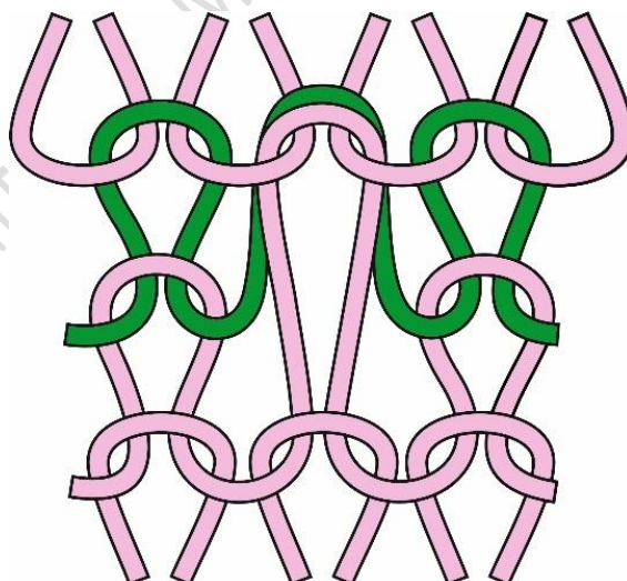
Figure 1.16: Tuck Knit
