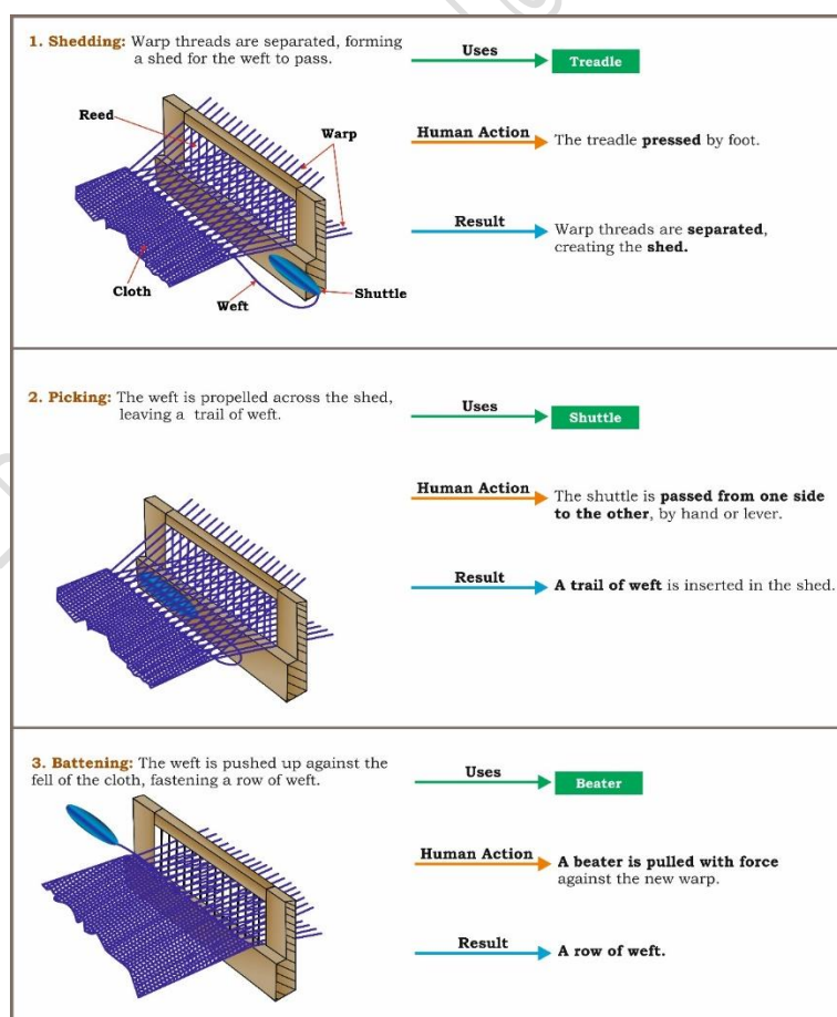
Figure 1.9: Process of Weaving
