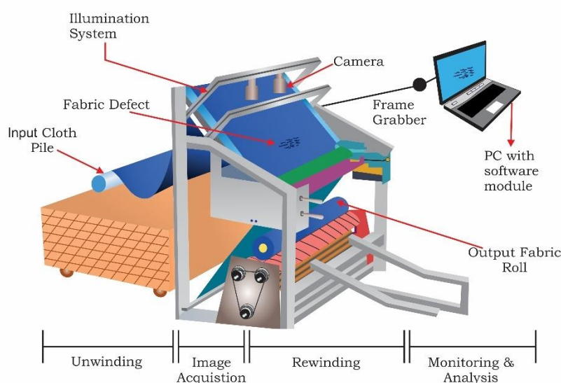
Figure 3.4: Process of an Automatic Fabric Inspection System
