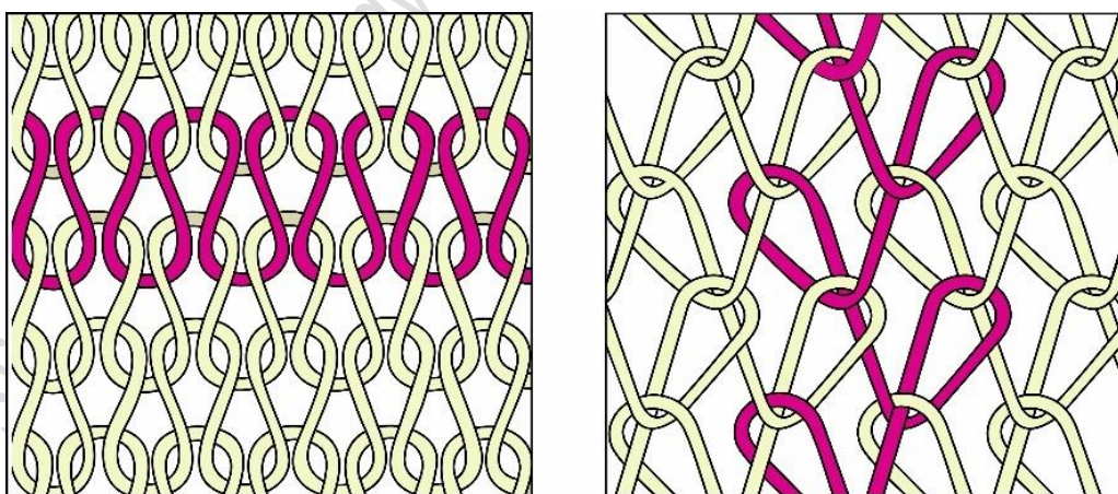
Figure 1.11: Weft Knit
