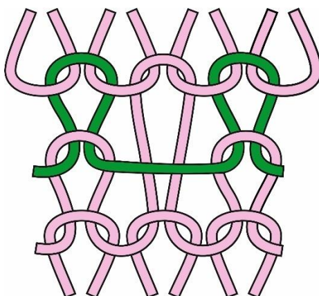
Figure 1.17: Missed- stitch or Float stitch
